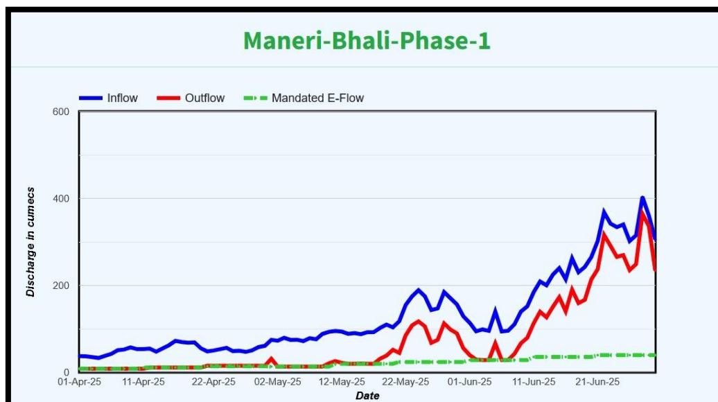
Figure 2: Graphs showing status of implementation of E-Flow at Maneri Bhali-I
