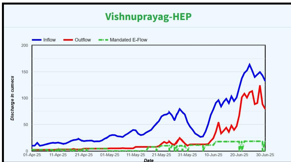
Figure 5: Graphs showing status of implementation of E-Flow at Vishnuprayag HEP
